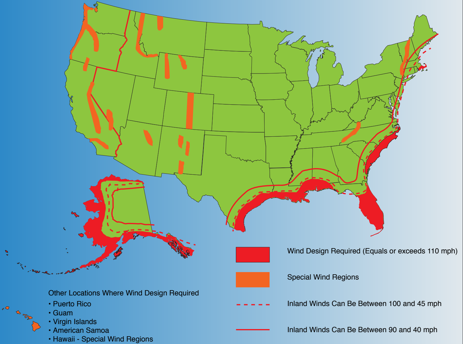
Regions Where Generator Canopy Design Must Manage Higher Wind Speeds
